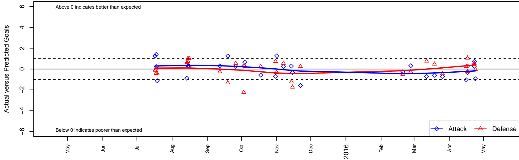
TC United Navy G03 Dots are actual minus expected GF (blue circles) and GA (red triangles). Blue line is smoothed change in attack strength. Red is smoothed change in defense strength.
